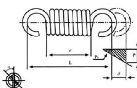
Tension
